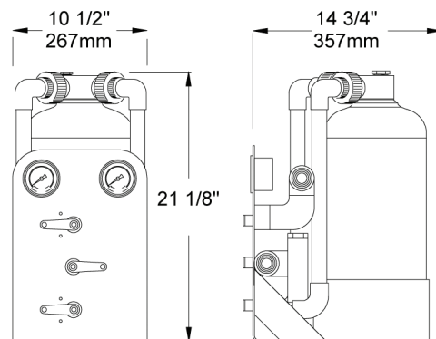
MULTI-MEDIA FILTER
