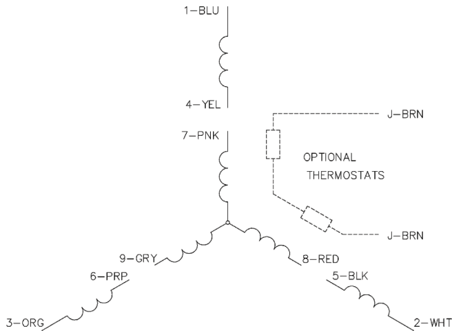
220 - 230 VAC LOW VOLTAGE (2Y)
