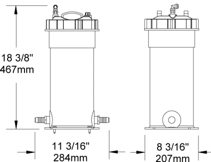
COMMERCIAL FILTER / OWS
