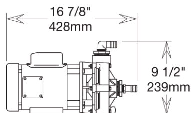
Booster Pump
