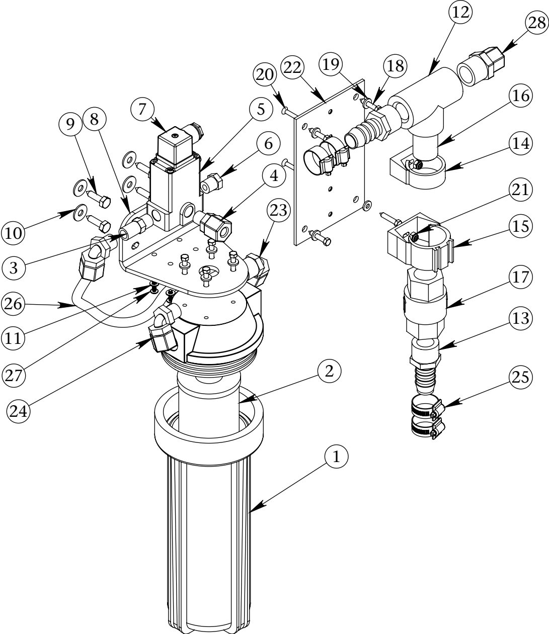
FRESH WATER FLUSH (.50 INCH) B598000008 - Illustration
