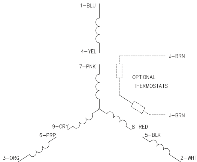
220 - 230 VAC LOW VOLTAGE (2Y)
