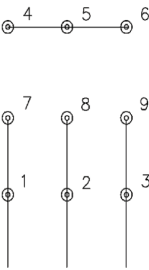
LINE LEADS 220 - 230 VAC
