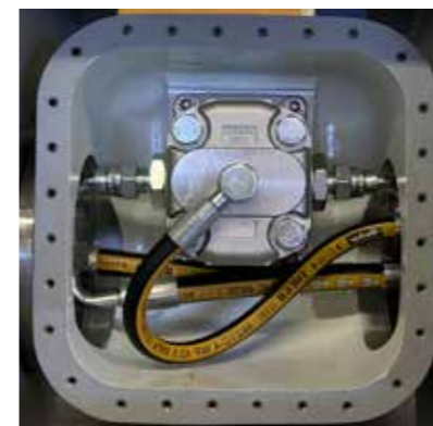
HYDRAULIC MOTOR
