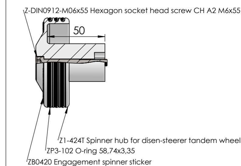
SP-DS-T Tandem spoke wheel
