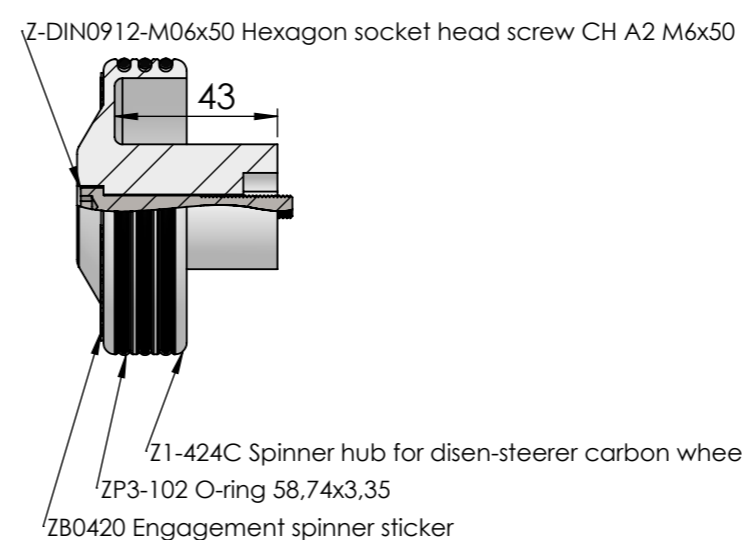
SP-DS-C Carbon wheel
